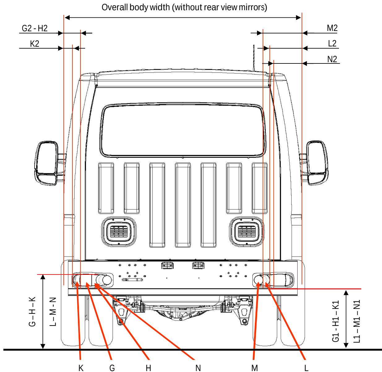
Rear lamps of chassis version
