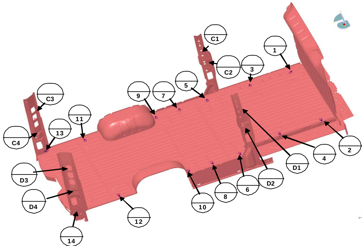
Panel Van L4, Rear Wheel Drive
