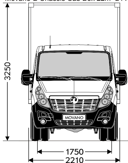
New Movano-B Chassis Cab Box 22m 3 L4 H1 RWD DRW
