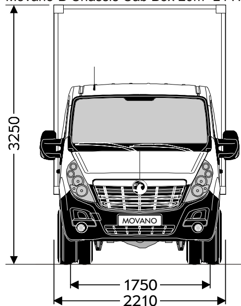
New Movano-B Chassis Cab Box 20m³ L4 H1 RWD DRW
