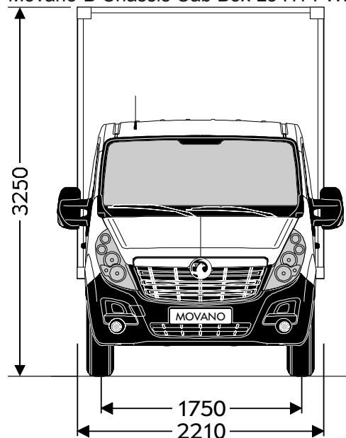
New Movano-B Chassis Cab Box L3 H1 FWD
