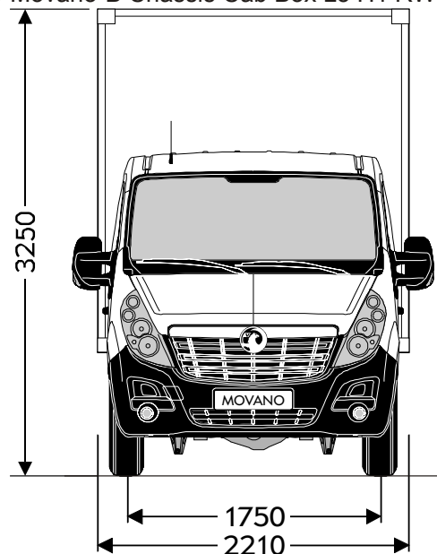
New Movano-B Chassis Cab Box L3 H1 RWD
