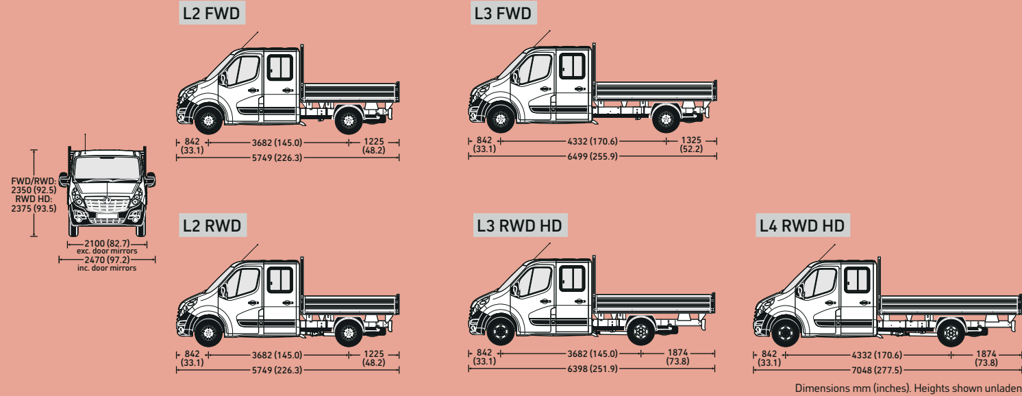
Dimensions mm (inches). Heights shown unladen.
