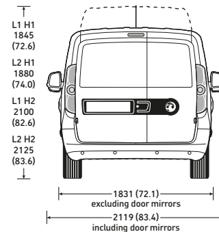
Dimensions mm (inches). Heights shown unladen.
