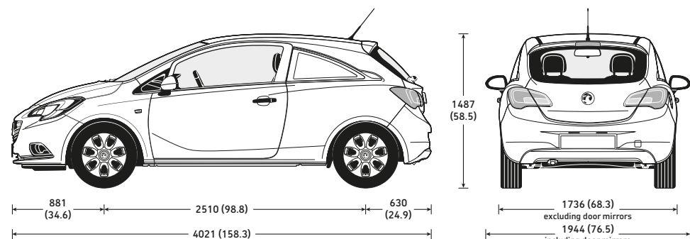
Dimensions mm (inches). Height shown unladen.
